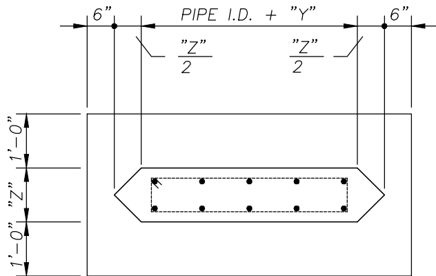
PLAN - IN STREAM
