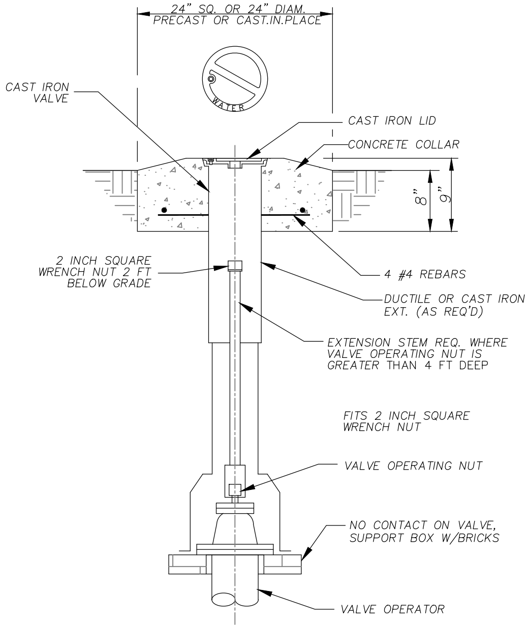
Underground Valve Box NTS
