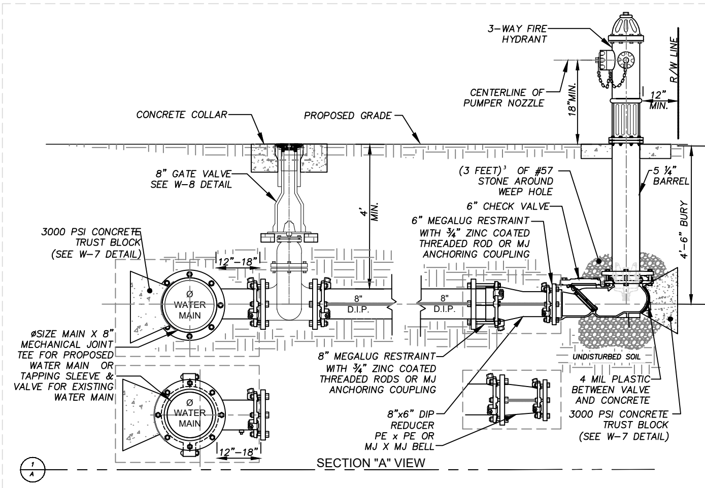
Fire Hydrant Assembled, 6" Check valve, 8" DIP branch and 8" Gate Valve
