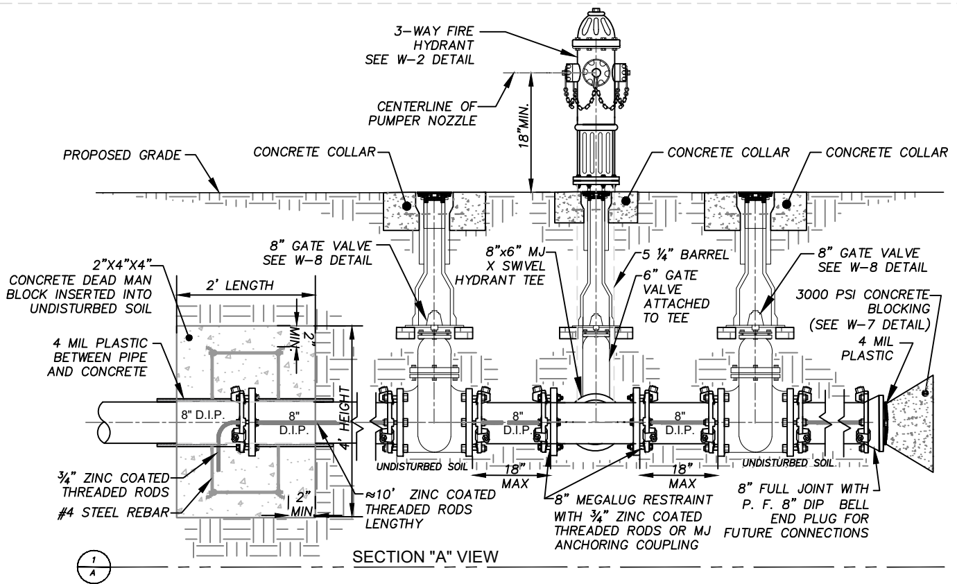
Dead End Fire Hydrant Assembled w/ Tee and Tee, Gate Valve for Future Extension
