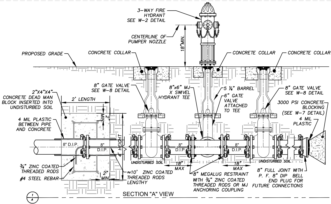
Dead End Fire Hydrant Assembled w/ Tee and Tree Gate Valve for Future Extension
